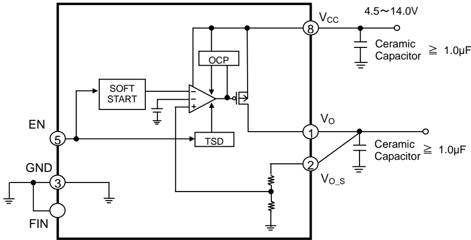
Figure 2. Block Diagram (Fixed type)
