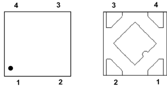
Top View X2-DFN1010-4 Bottom View
