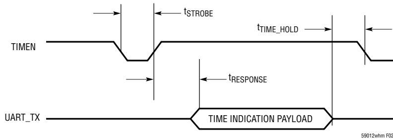
Figure 2. Timestamp Timing
