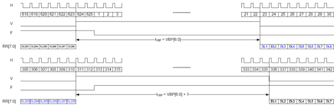
CCIR656 Vertical Timing
