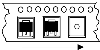
TO252 - 263 Package Orientation
