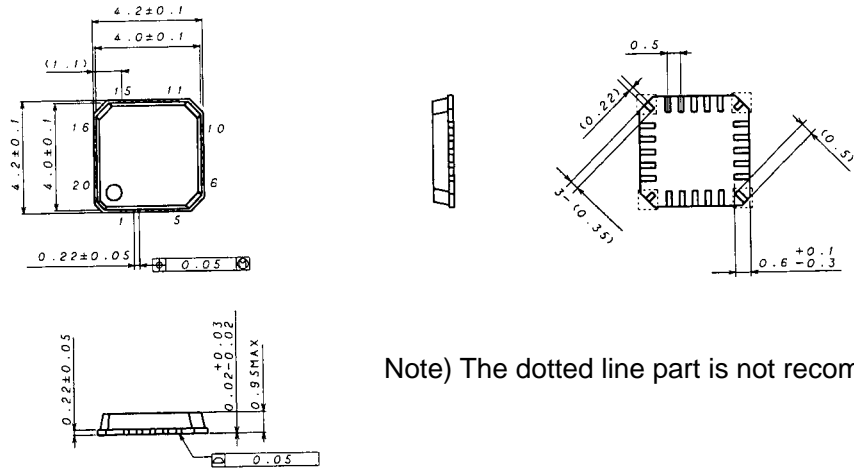
Fig.1 (Units:mm)
