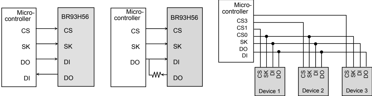
Figure 29-(a) Connection by 4 lines Figure 29-(b) Connection by 3 lines Figure 29-(c) Connection example of multiple devices Figure 29 Connection Methods with a Microcontroller
