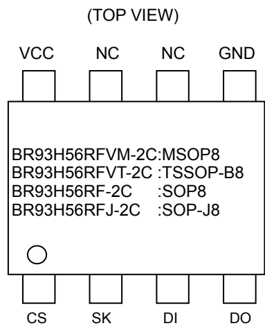
Figure 3 Pin Configuration
