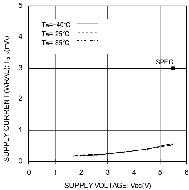
Figure 18. Supply Current (WRAL) vs Supply Voltage (fsk=3MHz)
