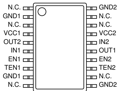
Figure 2. BM67221FV-C Package (SSOP-B20W)
