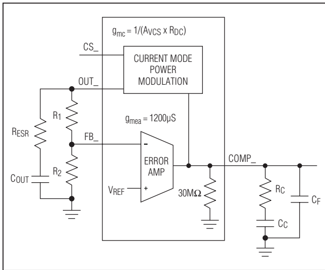
Figure 2. Compensation Network
