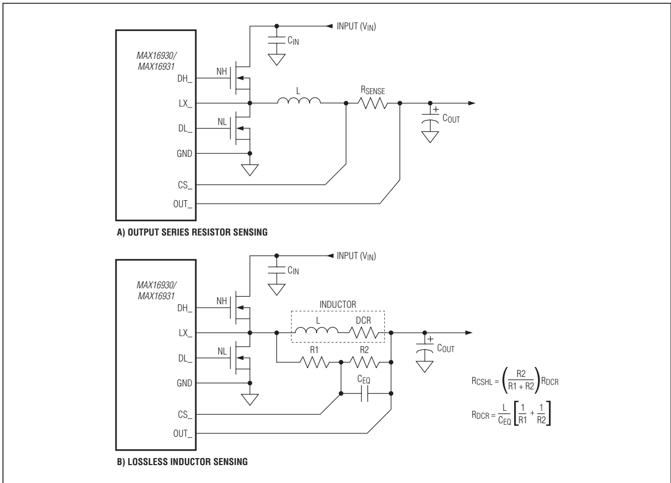
Figure 1. Current-Sense Configurations
