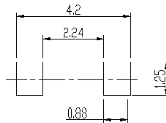
Soldering footprint
