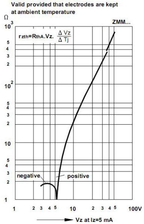
Thermal differential resistance versus Zener voltage
