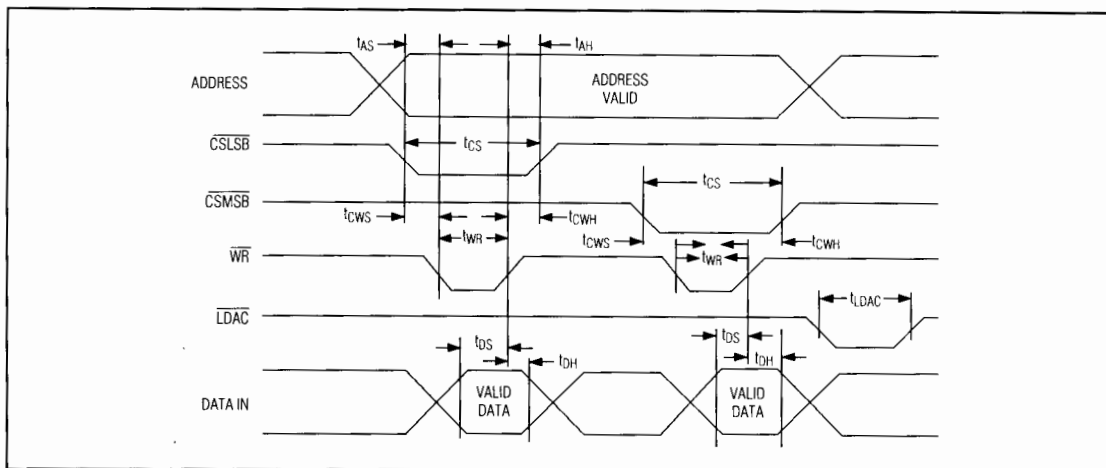
Figure 3. Write-Cycle Timing
