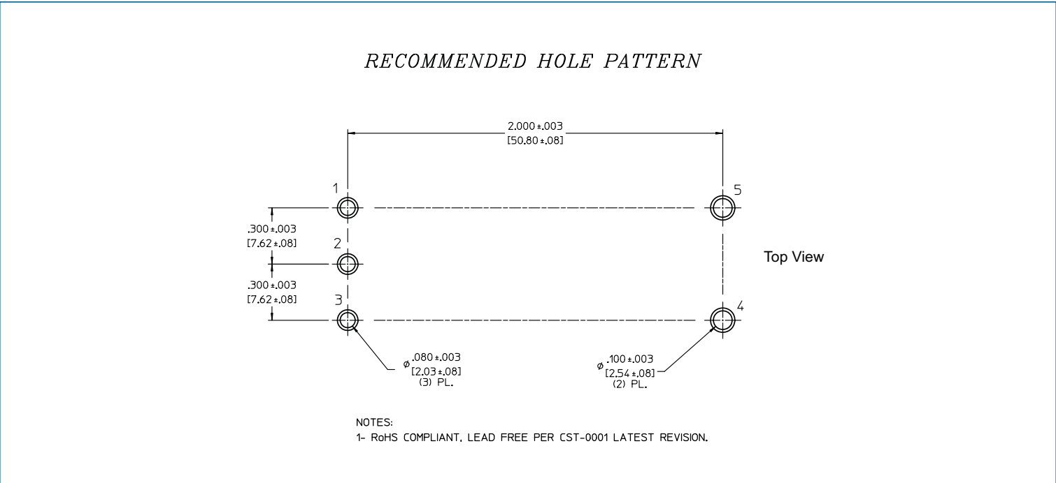
Figure 33 — IBC PCB recommended hole pattern
