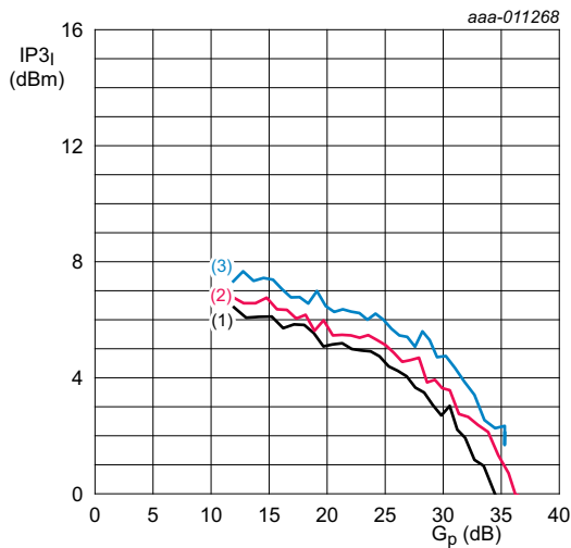
GS1 = LOW; GS2 = HIGH; V_{CC1} = 5\text{ V} ; V_{CC2} = 5\text{ V} ; f = 1950\text{ MHz} . (1) T_{amb} = -40\text{ }^{\circ}\text{C} (2) T_{amb} = +25\text{ }^{\circ}\text{C} (3) T_{amb} = +85\text{ }^{\circ}\text{C}
