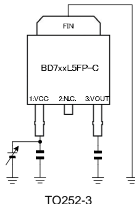
Figure 2. Typical Application Circuits
