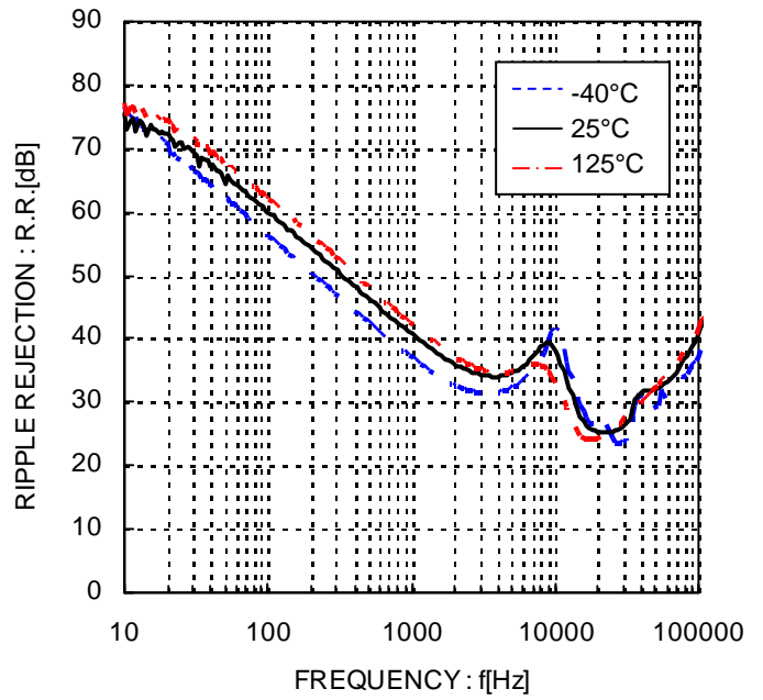
Figure 10. Ripple rejection (ein=1Vrms, IOU=100mA)
