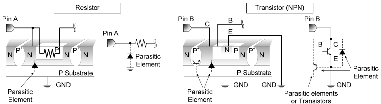
Figure 26. Example of the Parasitic Device Structures
