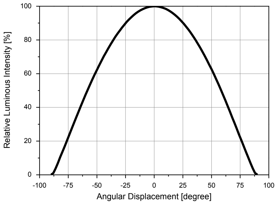
Fig 2. Radiant pattern, I_F=20\text{mA} , T_J=25^\circ\text{C}
