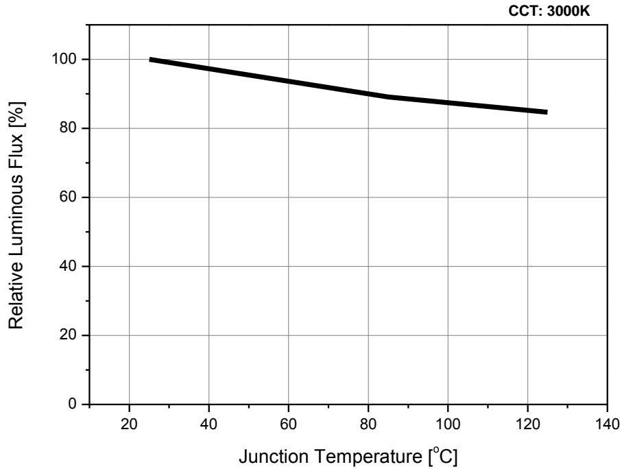
Fig 5. Relative Light Output vs. Junction Temperature, I_F=20\text{mA}
