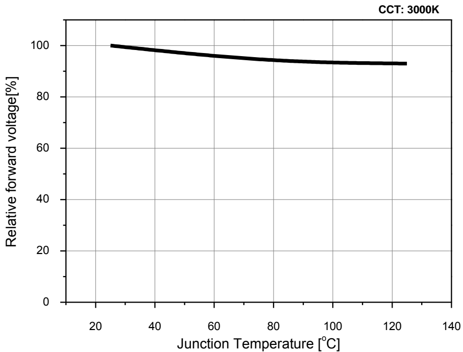
Fig 6. Forward Voltage vs. Junction Temperature, I_F=20\text{mA}
