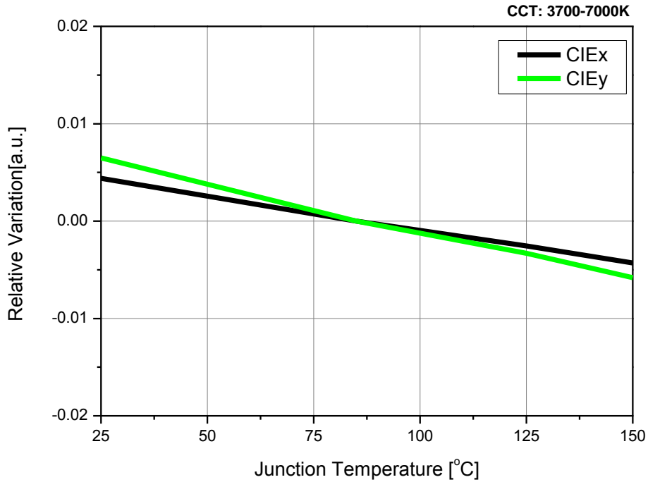
Fig 8. Junction Temperature vs. CIE x, y Shift, I_F=20mA
