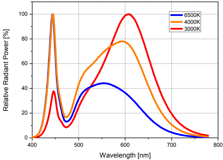
Fig 1. Color Spectrum, I_F=20\text{mA} , T_J=25^\circ\text{C}
