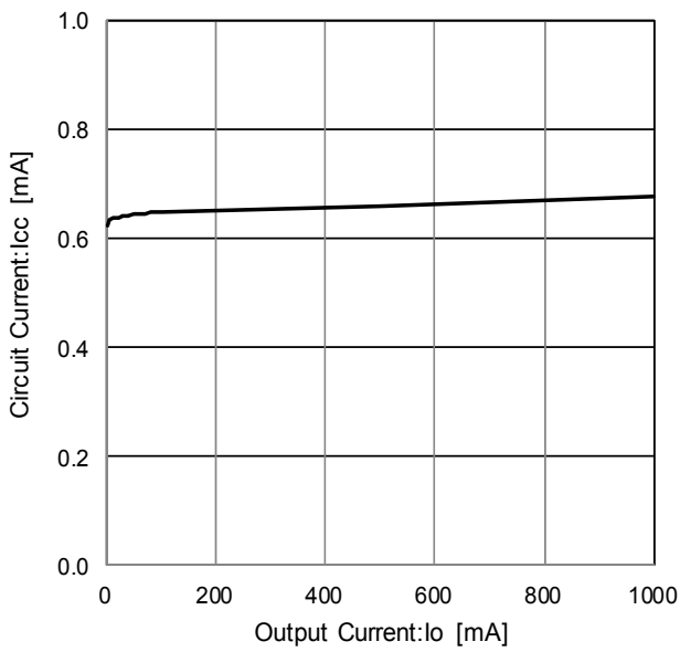
Figure 55. Circuit Current
