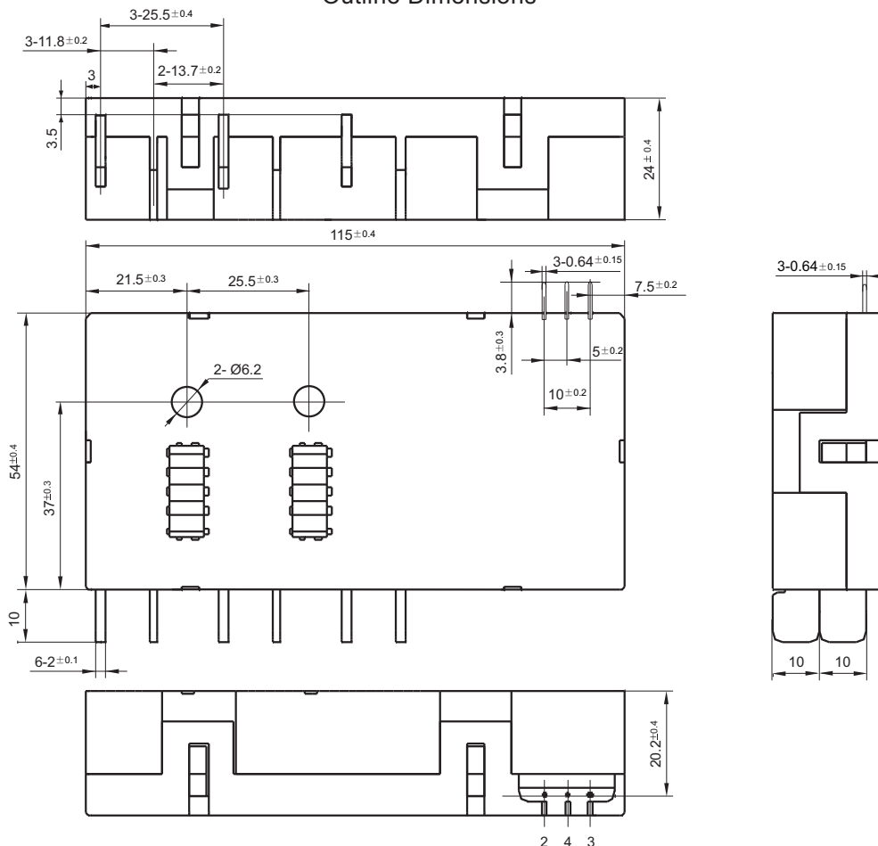
Outline Dimensions
