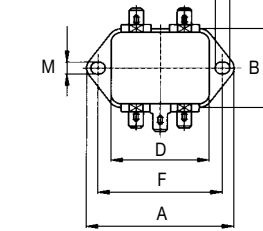
Housing F2
