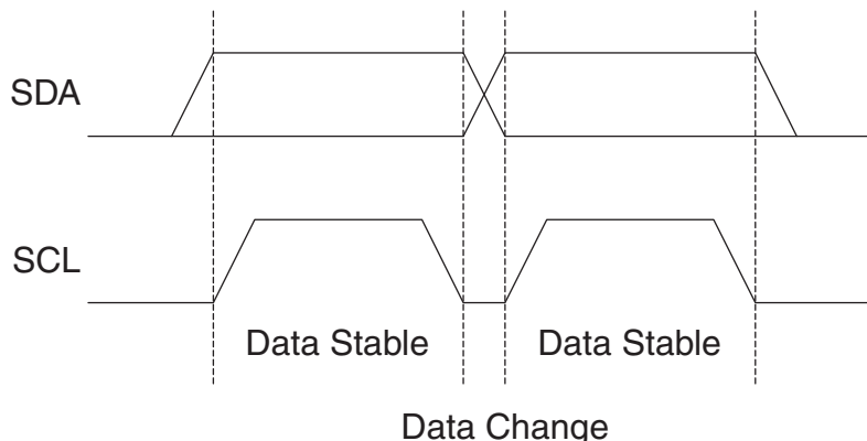
Figure 19-2. Data Validity
