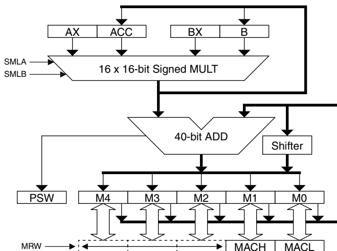
Figure 5-3. Multiply–Accumulate Unit
