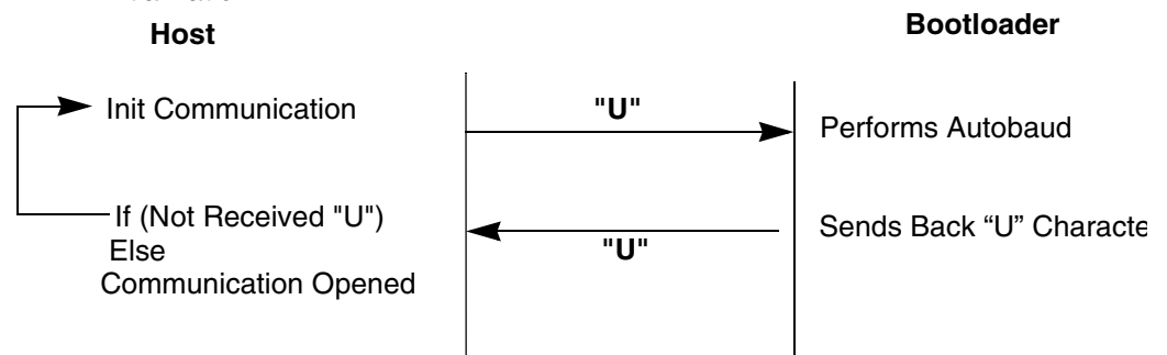
Figure 24-11. Initialization
