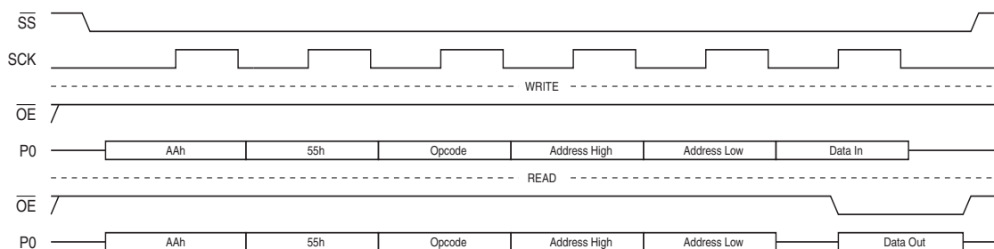
Figure 24-21. ISP Command Packet (Parallel)
