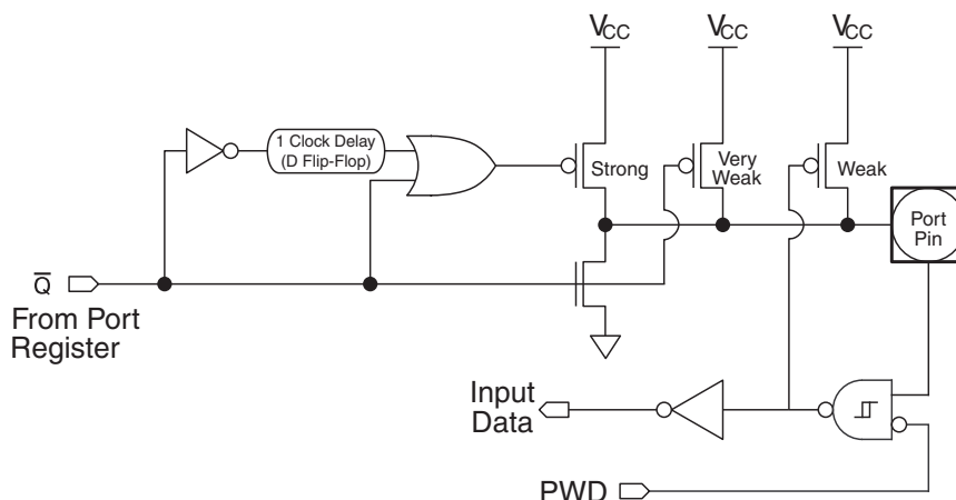
Figure 12-1. Quasi-bidirectional Output
