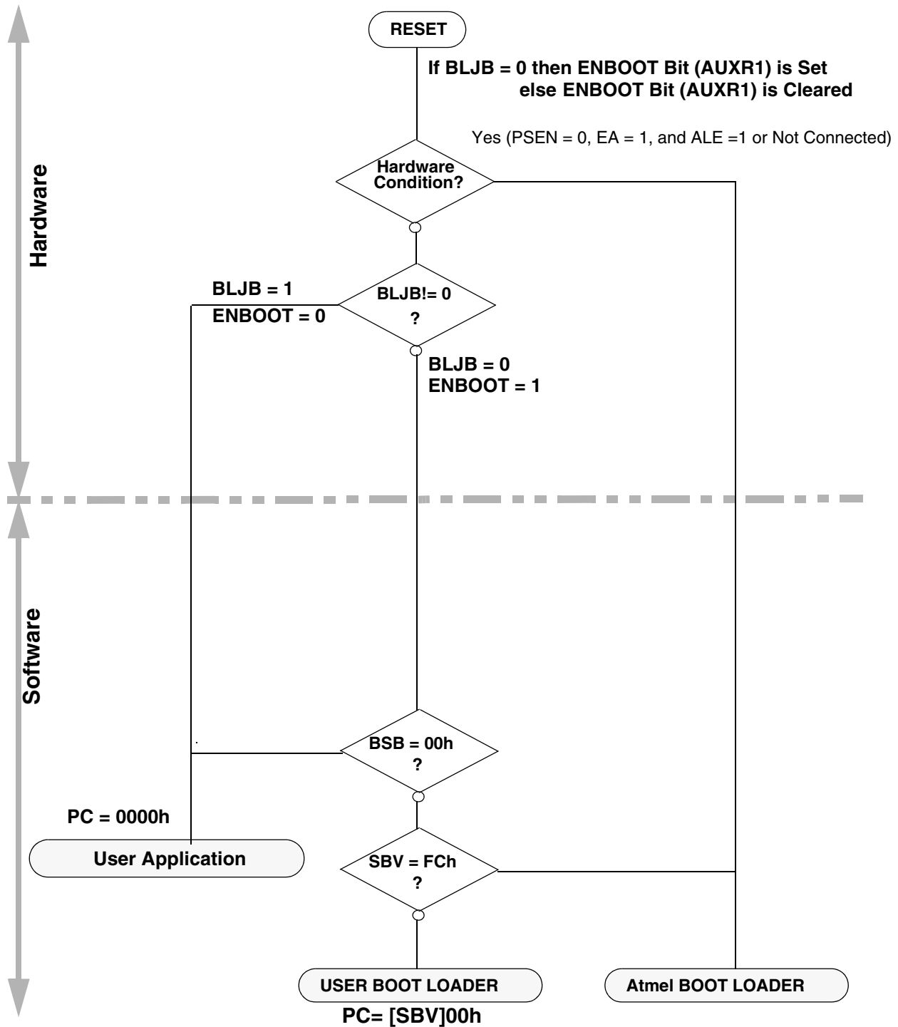
Figure 24-9. Bootloader Process
