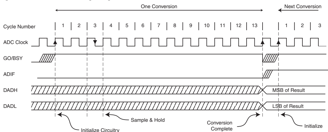
Figure 21-3. ADC Timing Diagram
