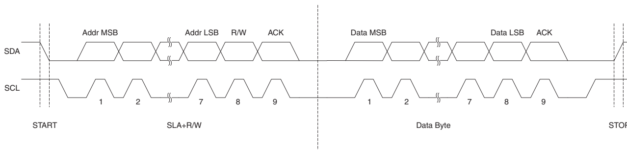
Figure 19-6. Typical Data Transmission
