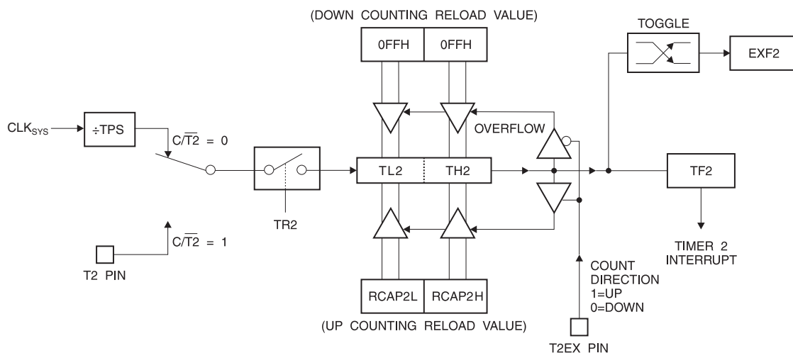
Figure 14-5. Timer 2 Diagram: Auto-Reload Mode (DCEN = 1)
