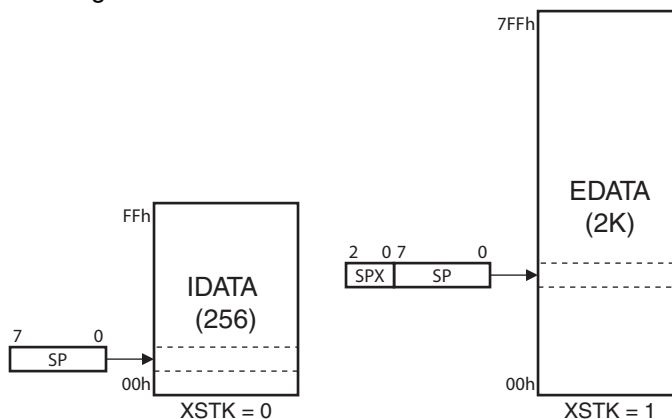
Figure 3-16. Stack Configurations
