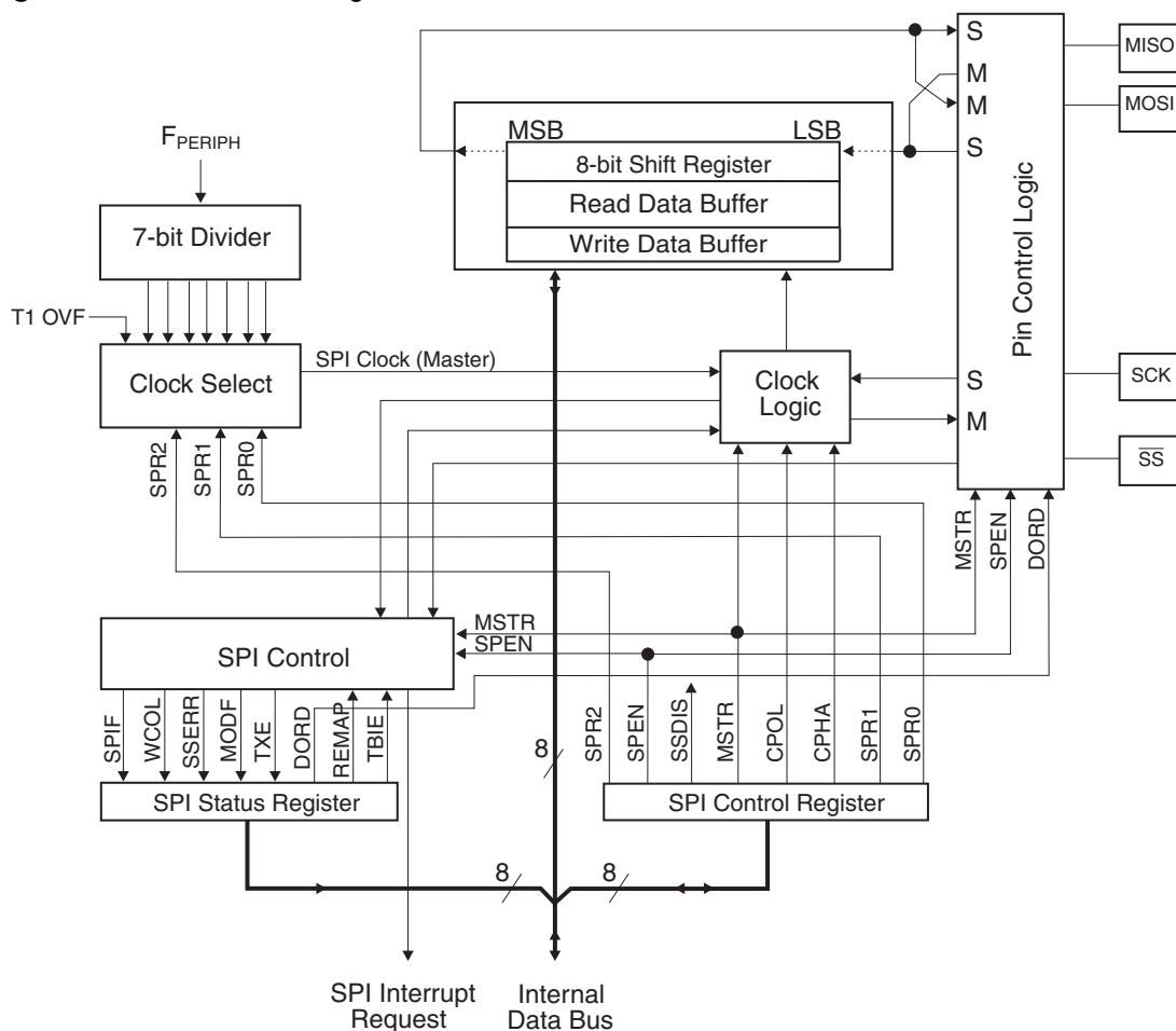
Figure 18-1. SPI Block Diagram
