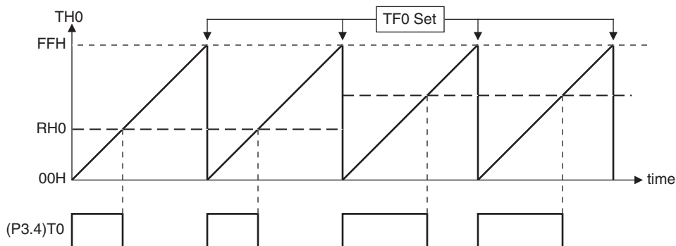
Figure 13-5. 8-bit Asymmetrical Pulse Width Modulation
