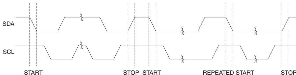
Figure 19-3. START, REPEATED START, and STOP Conditions
