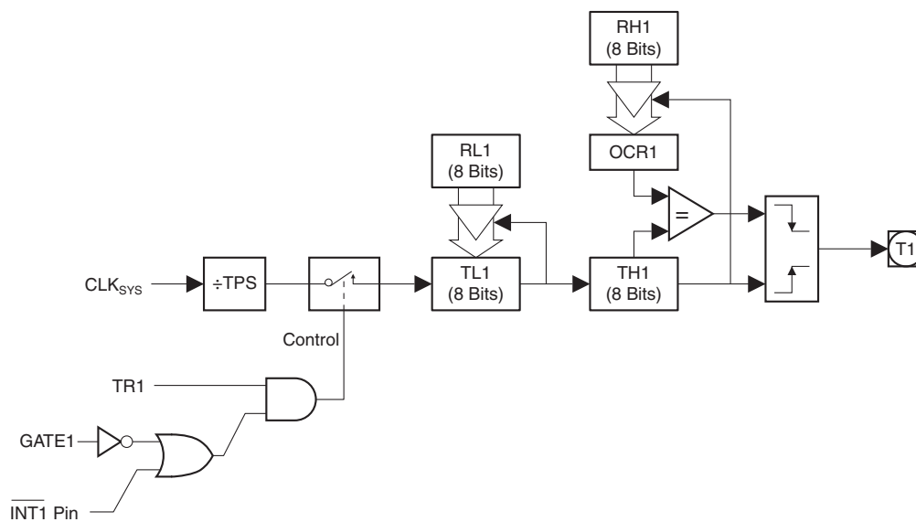
Figure 13-7. Timer/Counter 1 PWM Mode 1
