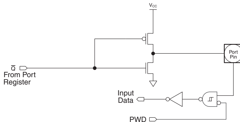
Figure 12-5. Push-pull Output
