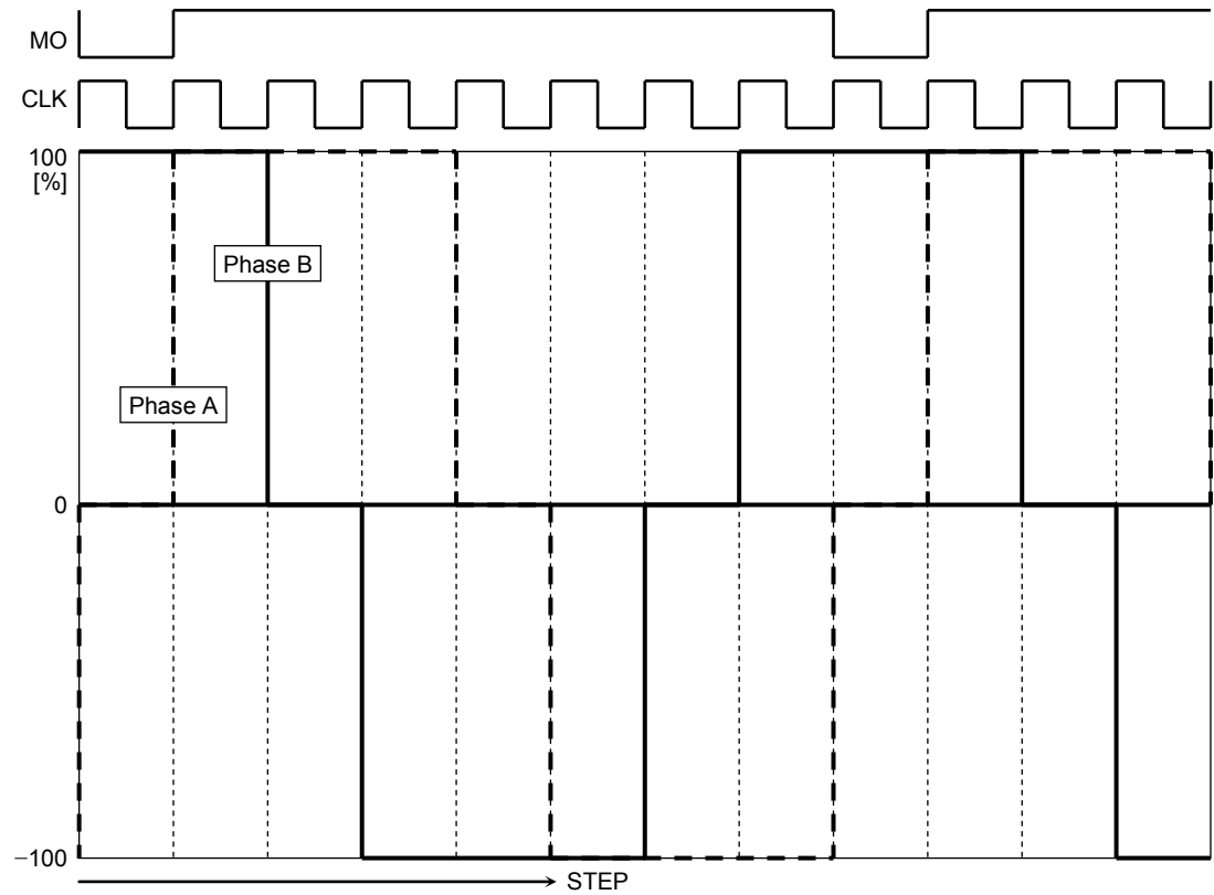
(4) 1-2 Phase Excitation mode (a)
