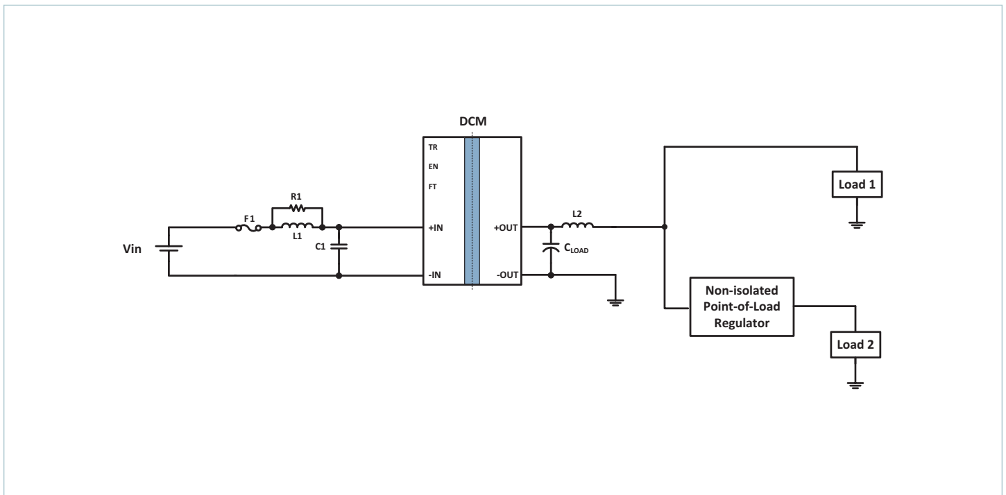
Typical Application 2: Single DCM48AP050x160A50, to a non-isolated regulator, and direct to load
