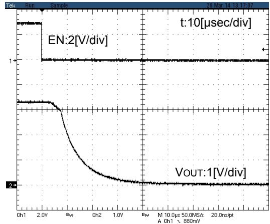
Figure.57 Turn off response 11 (BUS1DJC3GWZ VIN=3.3V)
