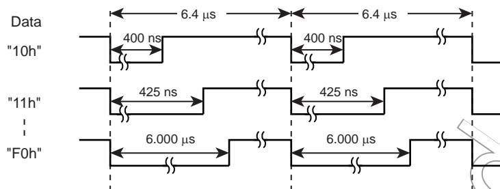
Figure 17-3 7-Bit Mode
