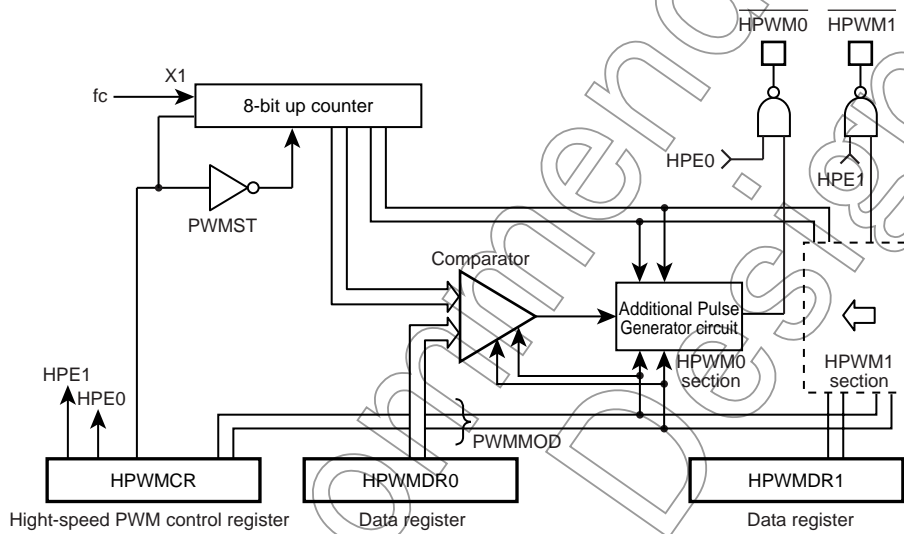
Figure 17-1 High-speed PWM (HPWM0 and HPWM1)
