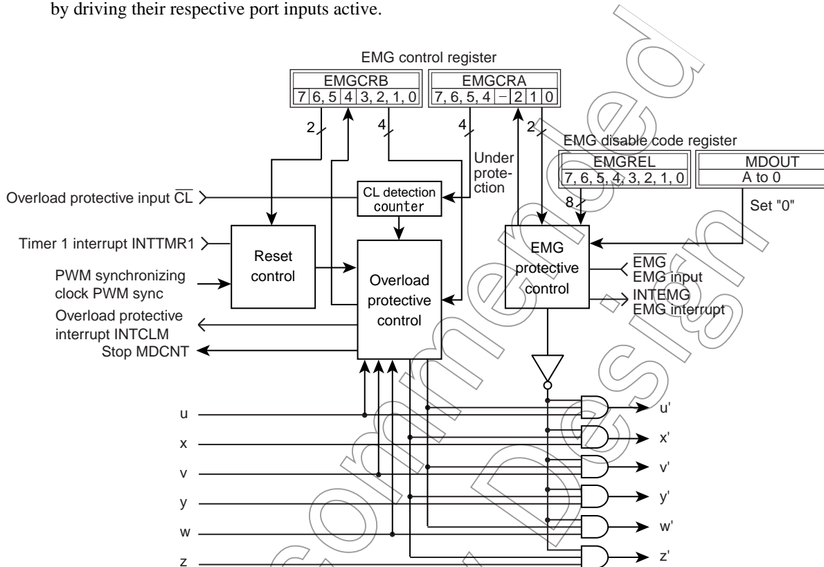
Figure 13-13 Configuration of the Protective Circuit
