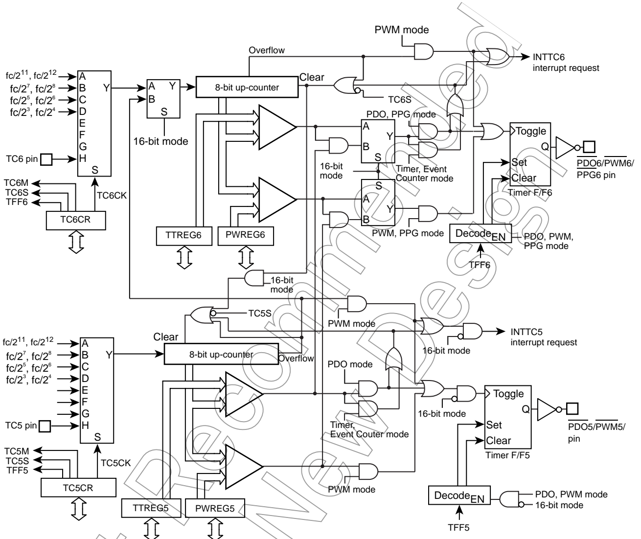
Figure 12-1 8-Bit TimerCounter 5, 6
