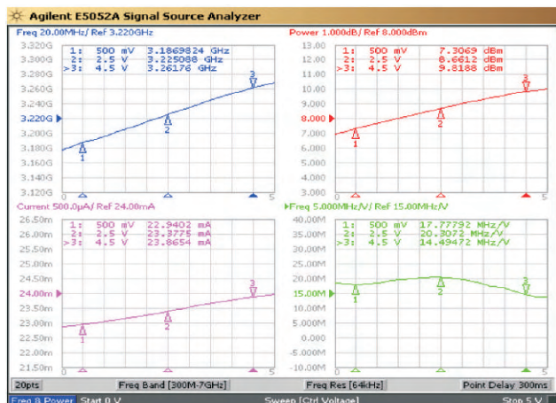
Frequency/power, tuning sensitivity, current of MCRO3228
