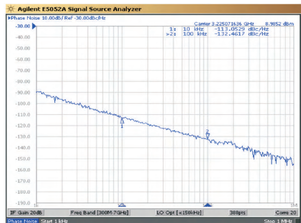
Phase noise of MCRO3228
