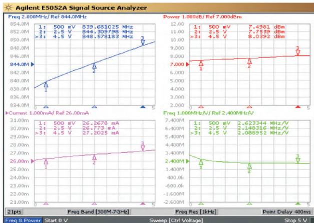
Frequency/power, tuning sensitivity, current of MCRO845
