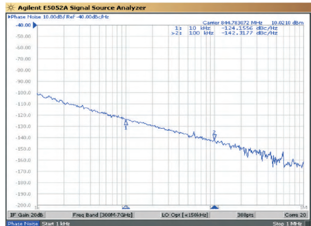
Phase noise of MCRO845
