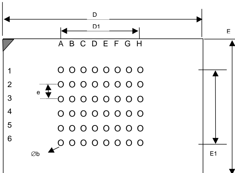
PACKAGE OUTLINE DWG.
