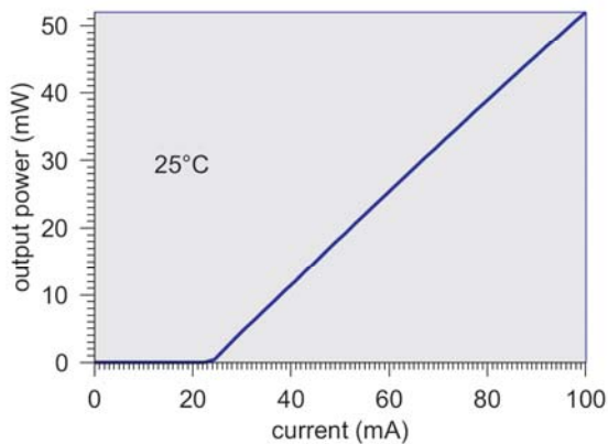
Current-Output-Power
