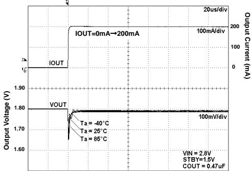
Fig 18. Load Response
