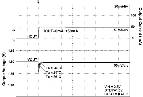
Fig 14. Load Response
