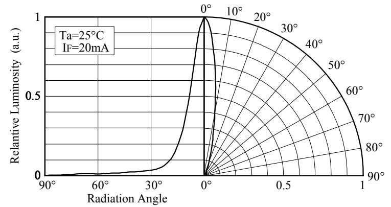
■ Directivity (NSPY500S)
