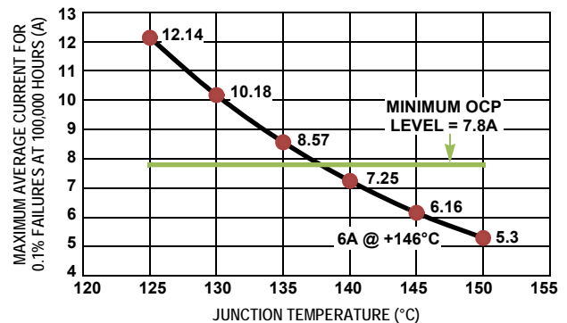
FIGURE 10. CURRENT vs TEMPERATURE
