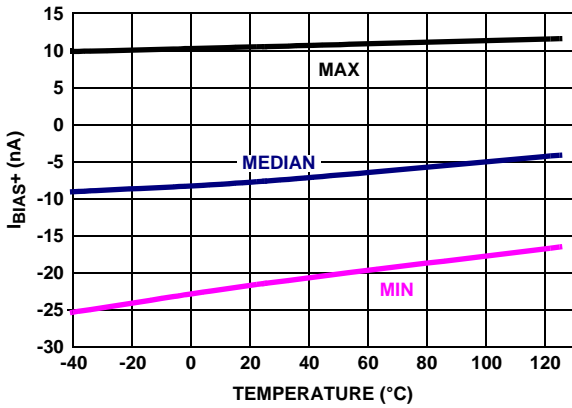
FIGURE 21. I_{BIAS+} vs TEMPERATURE, V_+, V_- = \pm 2.5V
