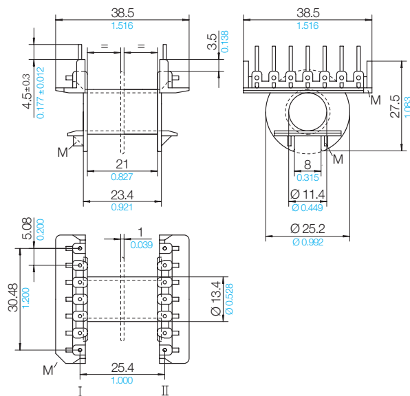
View pin-side
