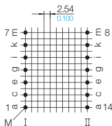
View pin-side
