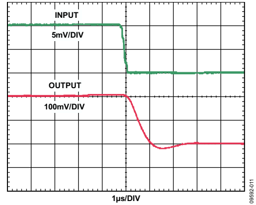
Figure 13. Fall Time (Differential Input = 10 mV)
