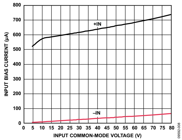
Figure 9. Input Bias Current vs. Input Common-Mode Voltage ( \text{Differential Input Voltage} = 5\text{ mV} , V_S = \text{NC} )
