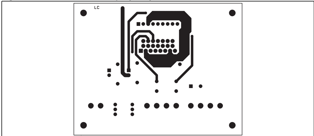
Figure 13. Reference board bottom layer layout
