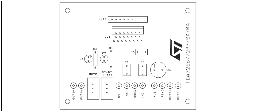
Figure 12. Reference board top layer layout
