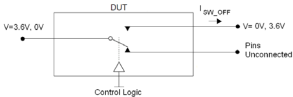
Figure 14. Off State Leakage
