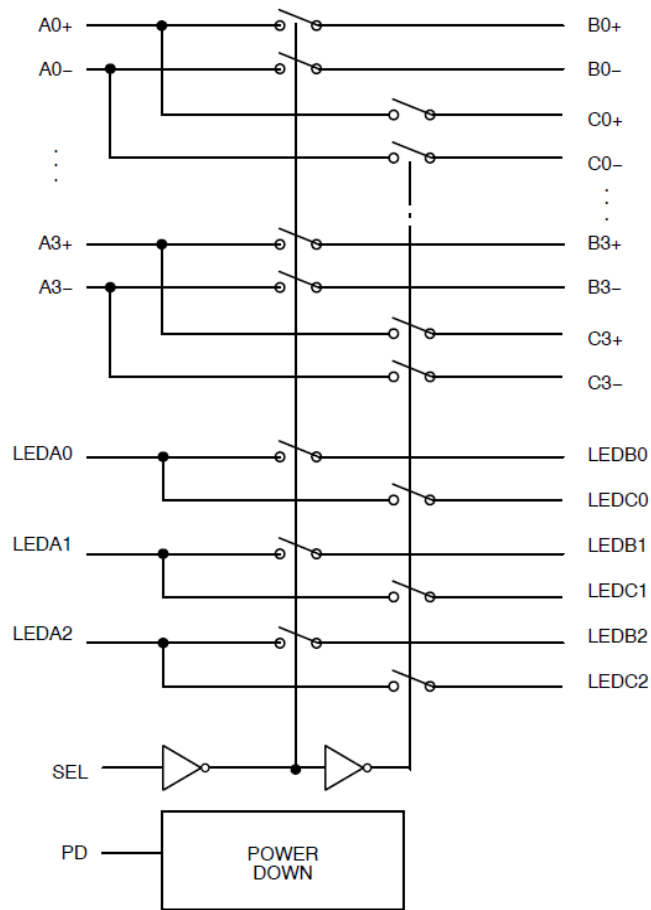
Figure 1. Block Diagram
