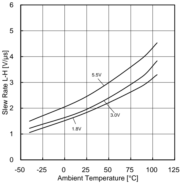
Figure 68. Slew Rate L-H vs Ambient Temperature
