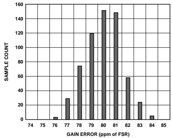
Figure 33. Gain Error Distribution Histogram (All Input Buffers Disabled, 647 Units)
