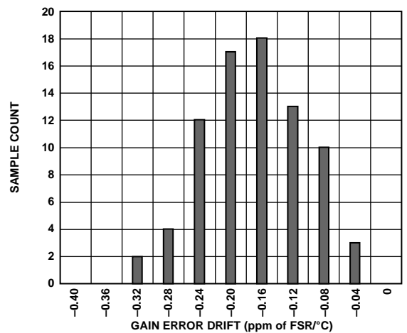
Figure 34. Gain Error Drift Distribution Histogram (All Input Buffers Enabled, 79 Units)
