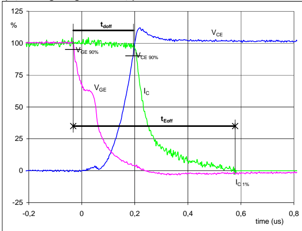
Figure 1 Buck IGBT
