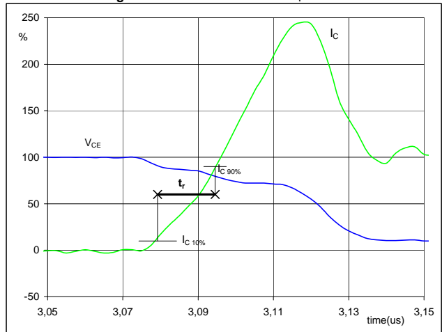
Figure 4 Buck IGBT
