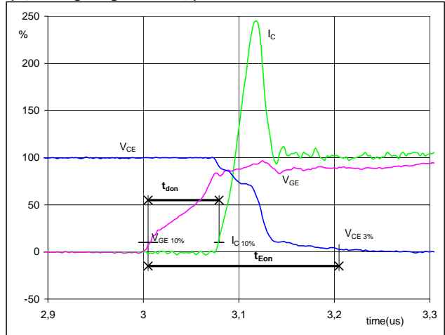
Figure 2 Buck IGBT
