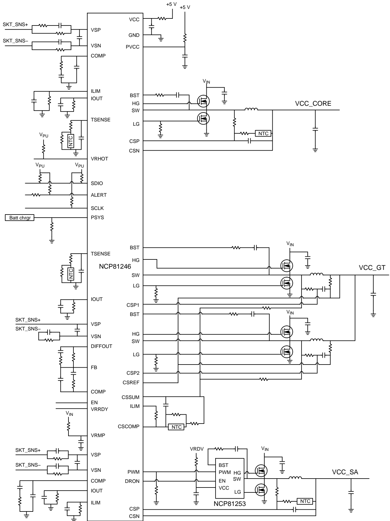
Figure 1. Application Schematic
