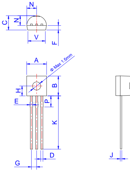
TO-92
