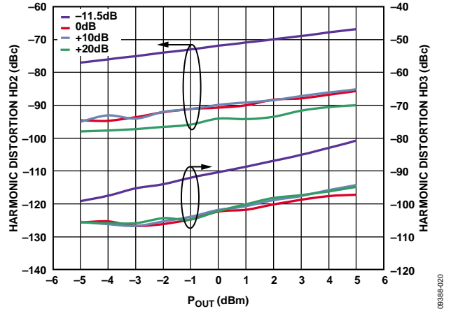
Figure 21. Harmonic Distortion vs. Power at Four Gain Codes, Frequency = 140 MHz
