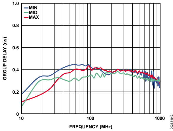
Figure 42. Group Delay vs. Frequency at Max, Mid, and Min Gain Outputs
