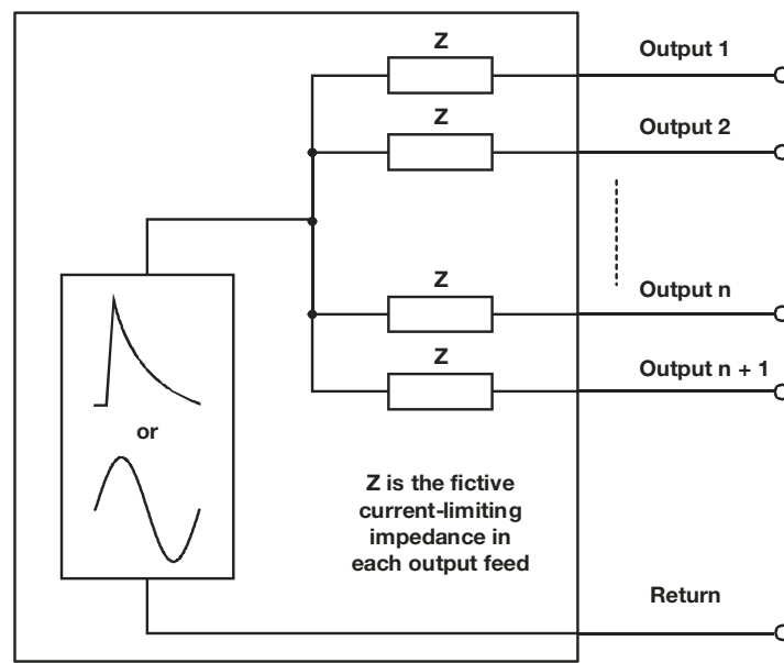
Generic Lightning or AC Test Generator
