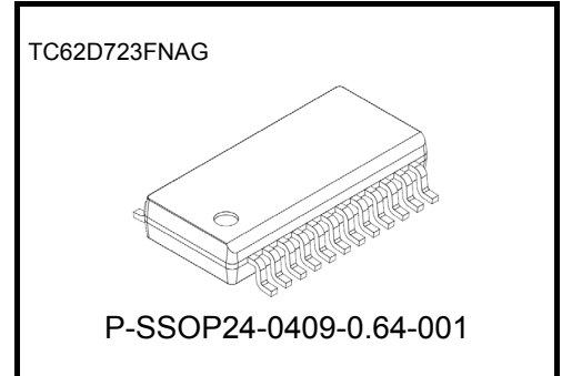
Weight P-SSOP24-0409-0.64-001:0.14g(Typ.)
