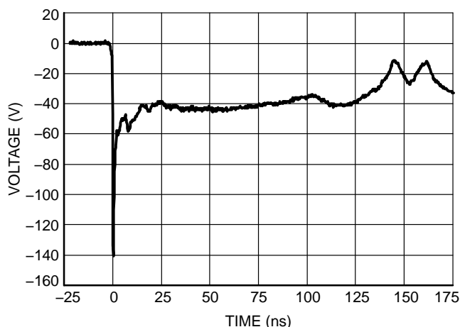
Figure 2. Typical IEC61000-4-2 - 8 kV Contact ESD Clamping Voltage
