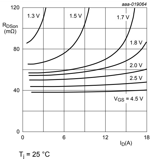
Fig. 9. Drain-source on-state resistance as a function of drain current; typical values T_j = 25 \text{ }^\circ\text{C}
