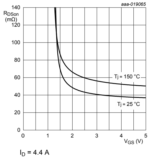
Fig. 10. Drain-source on-state resistance as a function of gate-source voltage; typical values I_D = 4.4 \text{ A}
