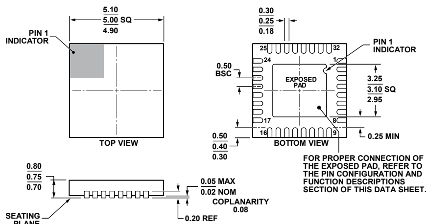
Figure 30. 32-Lead Frame Chip Scale Package [LFCSP_WQ] 5 mm x 5 mm Body, Very Very Thin Quad (CP-32-7) Dimensions shown in millimeters
