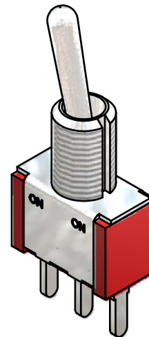
ISOMETRIC
