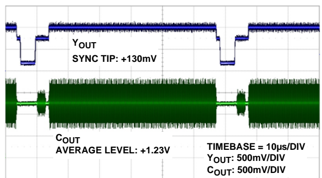
FIGURE 16. S-VIDEO OUTPUT
