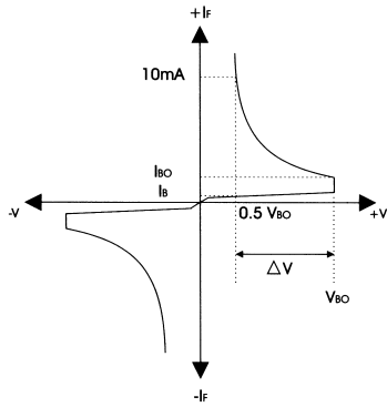
DIAGRAM 1: Current-voltage characteristics
